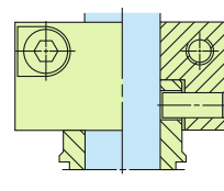
Clamping ring with pin
