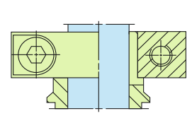
Clamping ring
