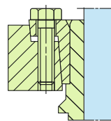
Shrink disk
