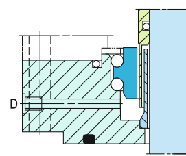
Option Polymerization barrier, can be used alternatively as a leakage drain or a flush.
