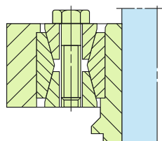
Clamping set
