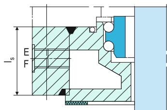
Option Cooling flange, can be used alternatively as a heating flange ( t_{max} = 350^{\circ}\text{C} (662 ^{\circ}\text{F} )).
