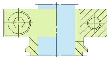
Clamping ring
