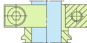
Clamping ring
