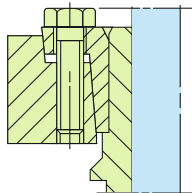
Shrink disc
