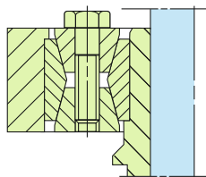
Clamping set
