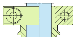
Clamping ring
