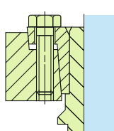
Shrink disk
